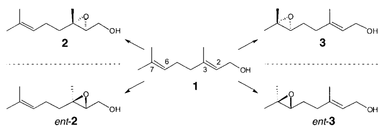
Scheme 1. Regio- and enantioselective monoepoxidations of geraniol.
